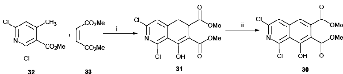
Scheme 7. Synthetic pathway for the compound 30 . Reagents and conditions: (i) LDA, THF, -78^{\circ}\text{C} , 45 min, then 33 , THF, -78^{\circ}\text{C} \rightarrow r.t, 12 h, 84%; (ii) DDO, benzene, reflux, 3 h.
