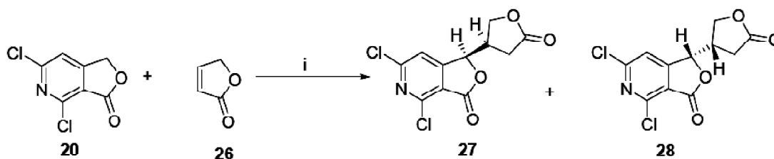
Scheme 5. Reaction of lactone 20 with lactone 26 . Reagents and conditions: (i) LDA, –60°C, → r.t, 12 h, 78%.
